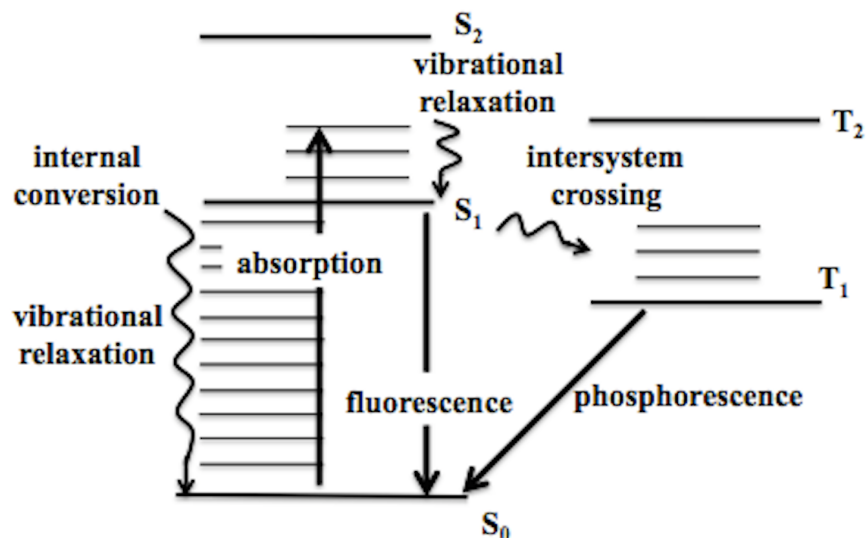
Figure 2.1. Simplified Jablonski diagram representing the photophysical processes possible for DOM.
