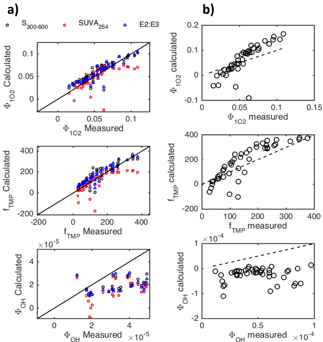
Figure E.11. Plots of calculated versus measured \Phi_{RI} for data from McCabe and Arnold (2016) with a one to one line shown for comparison. a) Calculations based on single linear regressions (developed with the dataset from the Florida Everglades) presented in Figure E.4. Legend indicates the regressor that was used in the model. b) Calculations based on multiple linear regressions (developed with the dataset from the Florida Everglades) presented in Figure E.10.
