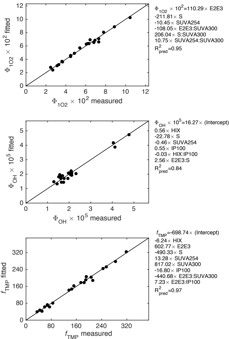
Figure E.8. Multiple linear regression models for all intrinsic predictors used in estimating RI quantum yields. The one to one line is shown for comparison. The fitted model equation and R^2_{\text{pred}} are shown for each \Phi_{\text{RI}} . Stepwise elimination was used to obtain only significant ( \alpha=5\% ) model terms.
