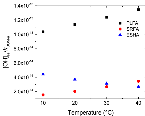
Figure D.6. Plot of steady state concentration of \bullet\text{OH} radical as a function of temperature due to both photochemical production of and scavenging by DOM. Note that the steady state concentration is normalized to the specific rate of light absorption.
