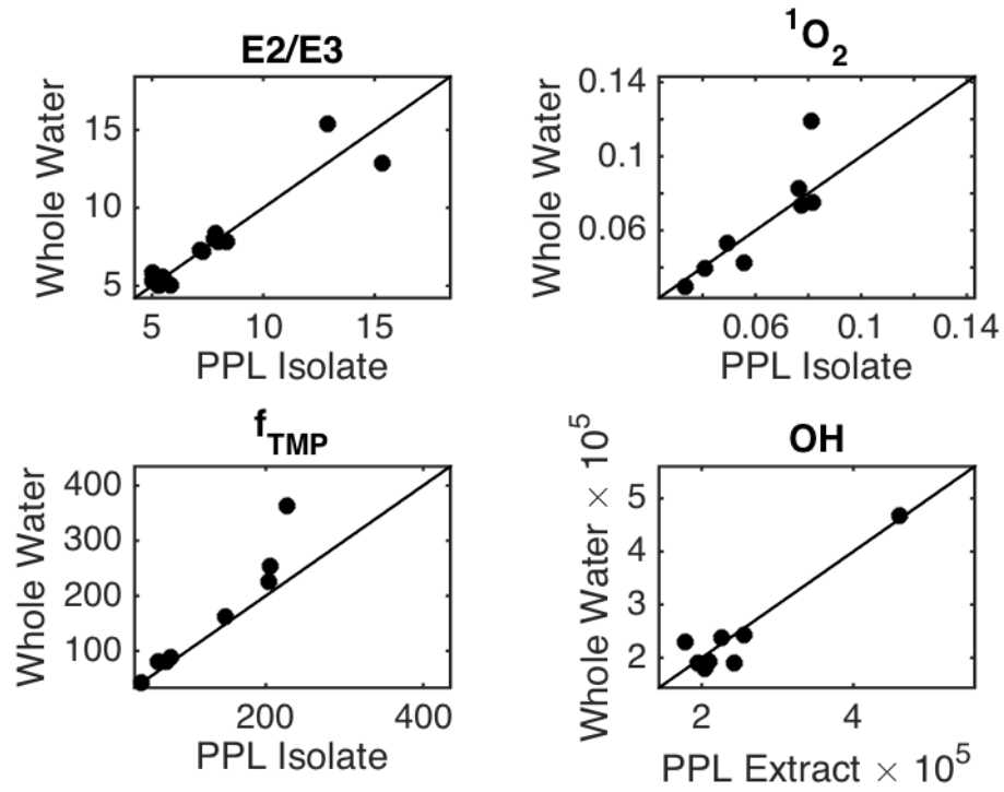
Figure E.12. Whole water versus PPL extract \Phi_{RI} values for select ( n=8 ) number of samples from this study. One to one line is shown for comparison.
