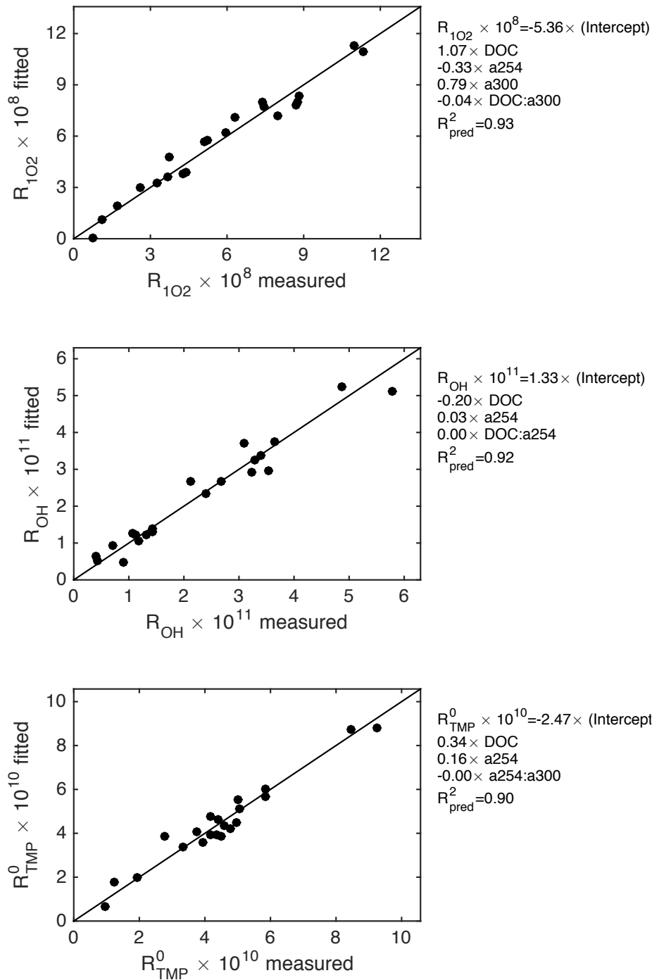
Figure E.6. Multiple linear regression models for the extrinsic predictors used in estimating RI formation rates. The one to one line is shown for comparison. The fitted model equation and R^2_{\text{pred}} are shown for each R_{\text{RI}} . Stepwise elimination was used to obtain only significant ( \alpha=5\% ) model terms.
