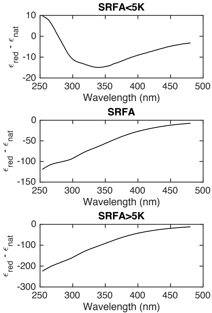
Figure A.10. Plot of \epsilon_{red} - \epsilon_{nat} for SRFA molecular weight fractions. Integration of the between the curve and \epsilon_{red} - \epsilon_{nat} = 0 gives the area for the metric provided in Table A.3 (row 3).
