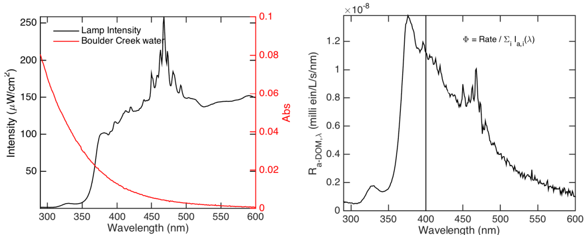
Figure E.2. (Left) Lamp spectra (black, left axis) for Oriell 94041 A solar simulator described in main text and absorbance spectra (red, right axis) for Boulder Creek non-base-modified. (Right) calculation of the rate of light absorption by DOM.
