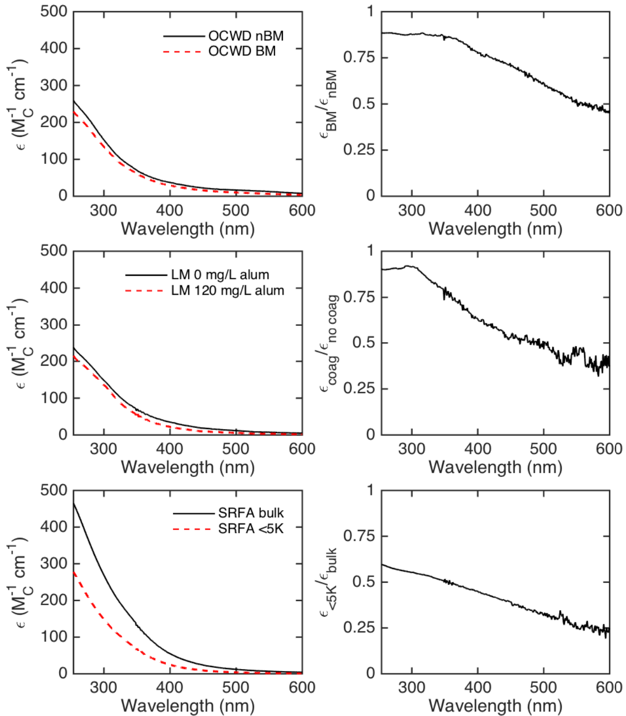
Figure 3.1. Carbon-based molar absorptivities plotted from 254 to 600 nm for wastewater samples and size-fractionated SRFA. (Right panels) Fraction of remaining absorptivity based on data in left panels. Absorbance scans collected with a 1 cm pathlength. [DOC] \sim 5-10 mg\ L^{-1} .
